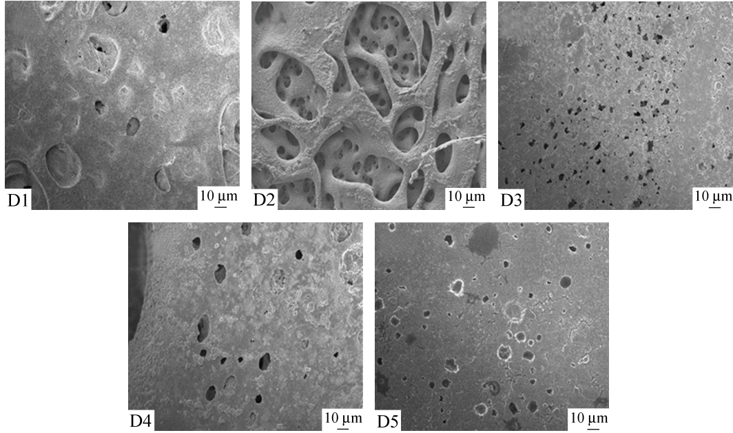
Fig. 8 Scanning electron microscope images of plasticized polymer electrolyte films containing (D1) PC, (D2) EC, (D3) GBL, (D4) DEC and (D5) DMC
